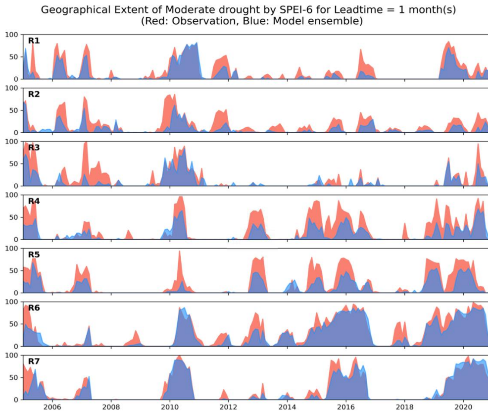
Figure 9. Geographical extent of Moderate drought by SPEI-6 for 1-month lead time. Red areas denote observed extent, while blue areas denote CTL predicted extent
