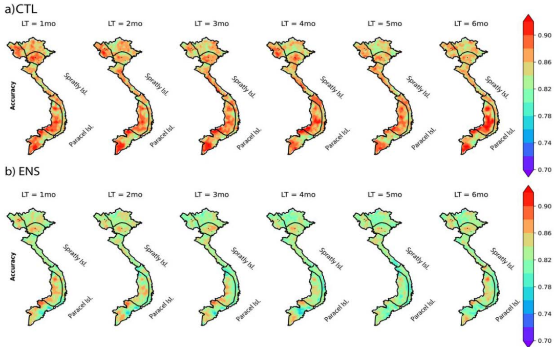
Figure 4. Accuracy index of (moderate and above) Drought Events categorized by SPEI-6 below -0.5
