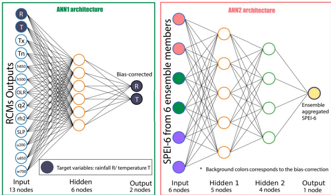
Figure 2. a-b) Schematic diagram of the hybrid model and experimental design (yellow boxes) and c) the Artificial Neural Network architectures designed in the drought forecasting procedure. In ANN1, the input nodes include rainfall R_{mod} , temperature T_{mod} , and various model outputs (see text for further descriptions); and the output nodes include bias-corrected R and T. In ANN2, the input layer includes SPEI-6 from the 6 ensemble members (background colors corresponds to the bias-correction), and the output includes ensemble aggregated SPEI-6 through neural network
