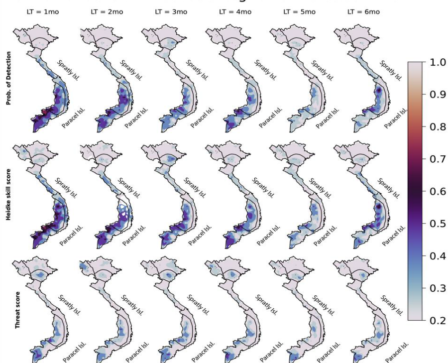
Verification scores of Moderate Drought Event Forecast in ENS
