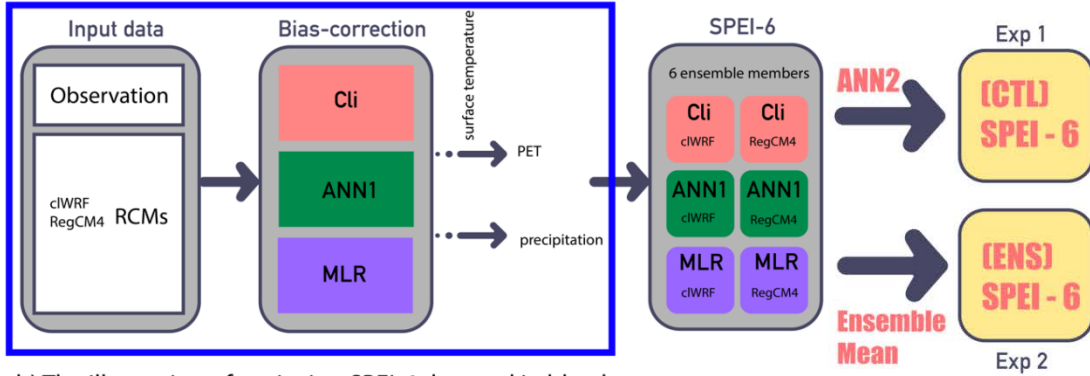
b) The illustration of retrieving SPEI-6 denoted in blue box
