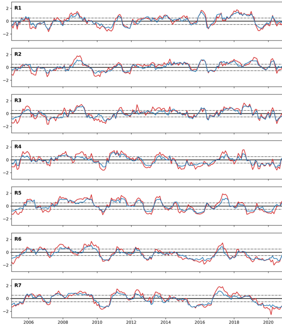
Figure 1. Evolution of the regional mean SPEI-6 for 1-month forecast by ENS model at different subregions in Vietnam. Dashed lines remark SPEI-6 at specific thresholds at -0.5 and 0.5
